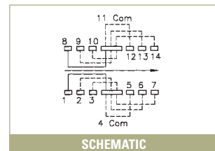
SCHEMATIC
