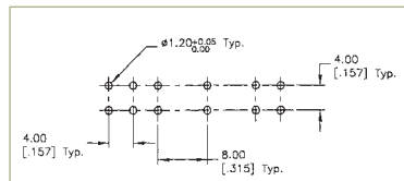
P.C. MOUNTING
