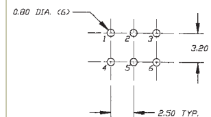
P.C. MOUNTING
