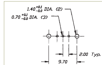
P.C. MOUNTING
