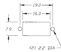
P.C. MOUNTING
