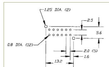
P.C. MOUNTING
